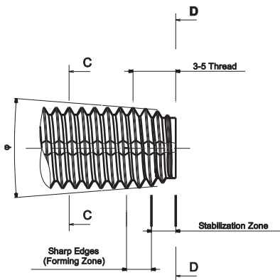
Basic dimensional specifications(mm)
